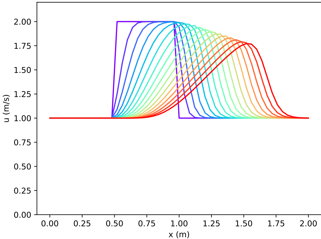
Figure 1: c=0.5\text{m/s} , nt=151 , nx=51 , t_{\text{max}}=0.5\text{s}
