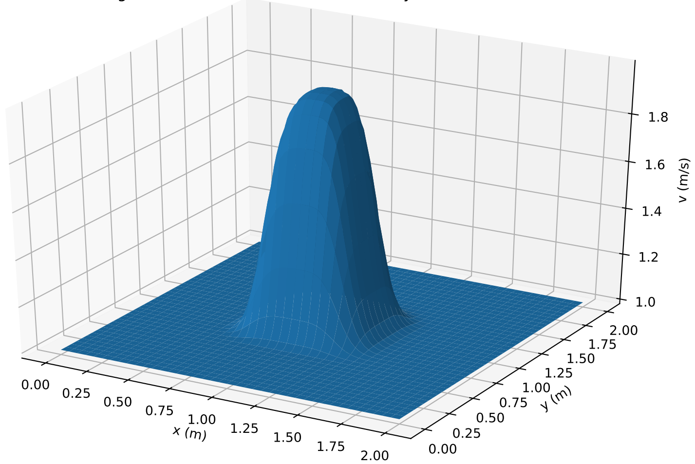
Figure 4: c=0.5\text{m/s} , nt=101 , nx=81 , ny=81 , t=0.5\text{sec}
